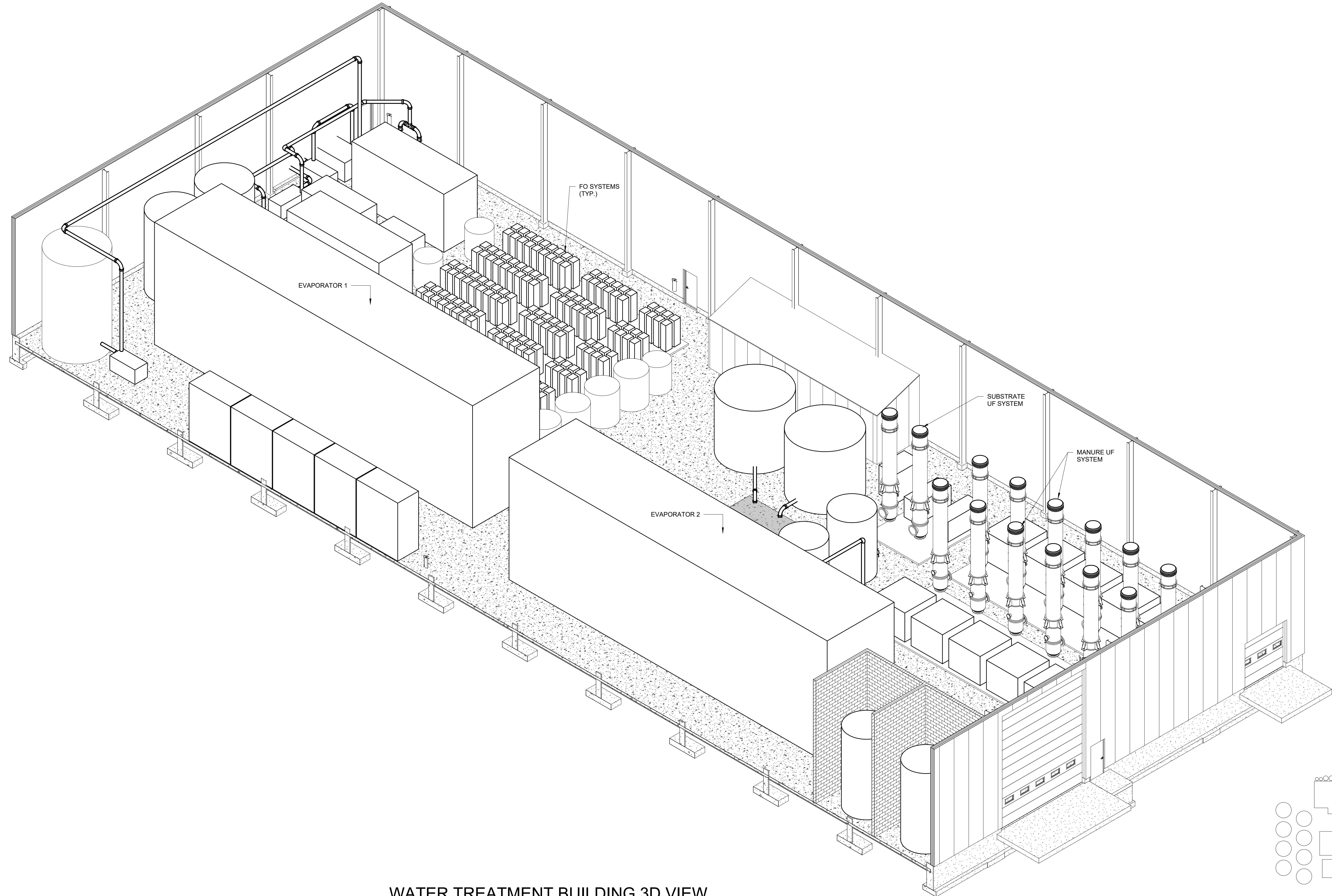
WATER TREATMENT BUILDING 3D VIEW NOT TO SCALE
